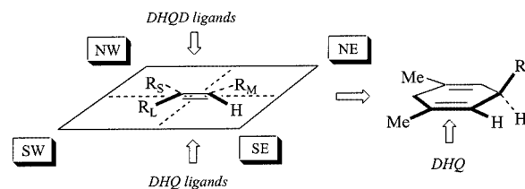
Figure 1. Quadrant method for rationalization of asymmetric dihydroxylation (AD) enantiofacial selectivity
